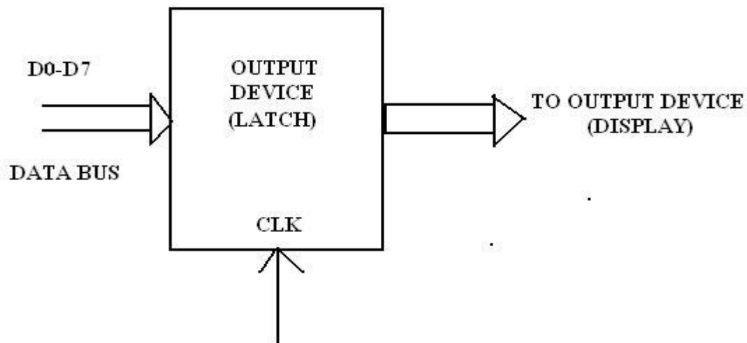
FIG.2 OUTPUT PORT
