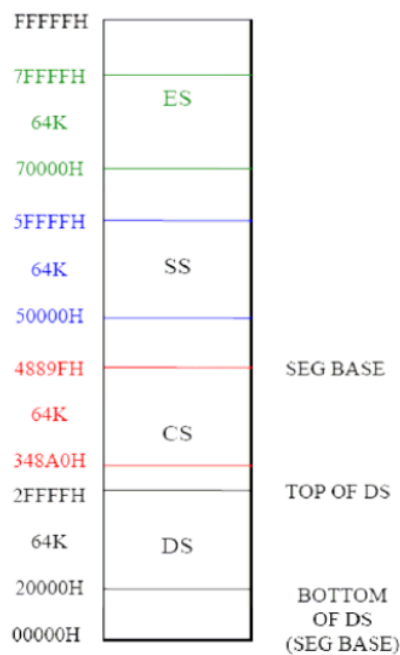
Fig1.5. Memory segmentation
